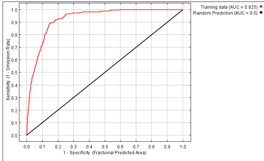
Fig. 6. ROC curve
